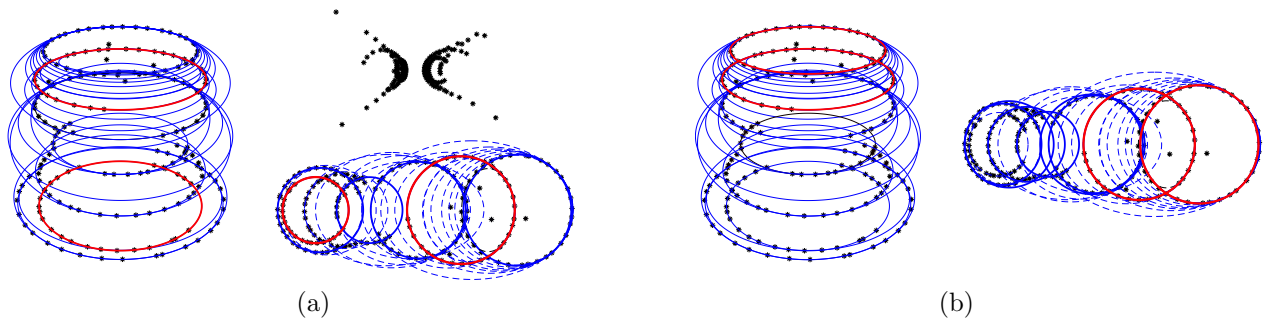
Figure 3. Example of Euclidean rectifications of a set of points V (black asterisks) from a pair of ellipses, highlighted in red, out of all the K_{\text{best}} ellipses (in blue) from the exhaustive search. Ellipses rectified in circles are shown in solid line, in dashed line otherwise. Red circles are the rectifications of the pair of ellipses used to compute the rectifications. (a) The two red ellipses (left) do not intersect, hence two rectifications are therefore computed from their intersections, namely from the two pairs of conjugate complex points. Top: no circle is found. Bottom: four ellipses, highlighted in blue, are rectified into circles. (b) When the red ellipses intersect into two real points, only one rectification is computed. Five ellipses are then rectified into circles. The ellipses rectified into circles are images of polyhedron trajectories.
