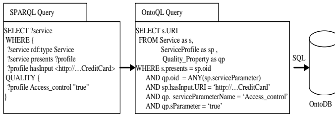
Fig. 7. Interpretation of the SPARQL QUALITY clause
