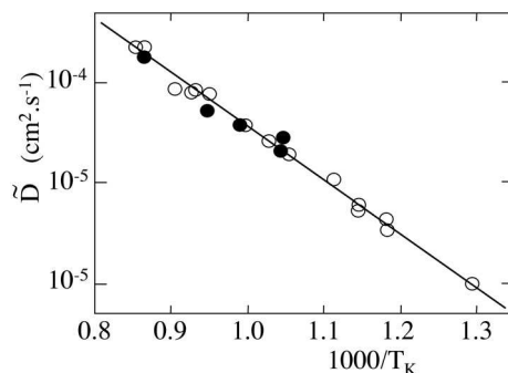
Fig. 23. Arrhenius plots of the oxygen chemical diffusion coefficient ( \tilde{D} ) measured on two samples with two different diffusion lengths: L_1 = 1.3\text{mm} ( \circ ) and L_2 = 0.7\text{mm} ( \bullet )
