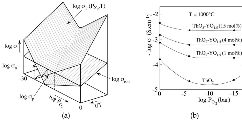
Fig. 17. (a): Schematic representation of \log \sigma surfaces over \log P_{O_2} , 1/T space for \sigma = \sigma_{ion} , \sigma_n , \sigma_p and \sigma_{total} , from [Patterson, 1971]; (b): \log \sigma vs. \log P_{O_2} for the system ThO_2-Y_2O_3 .
