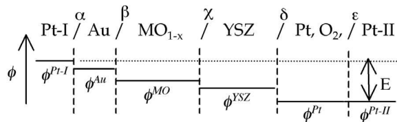
Fig. 5. Qualitative variation of the potential within the chain.
