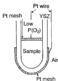
Fig. 10. Schematic diagram of the coulometric titration cell.
