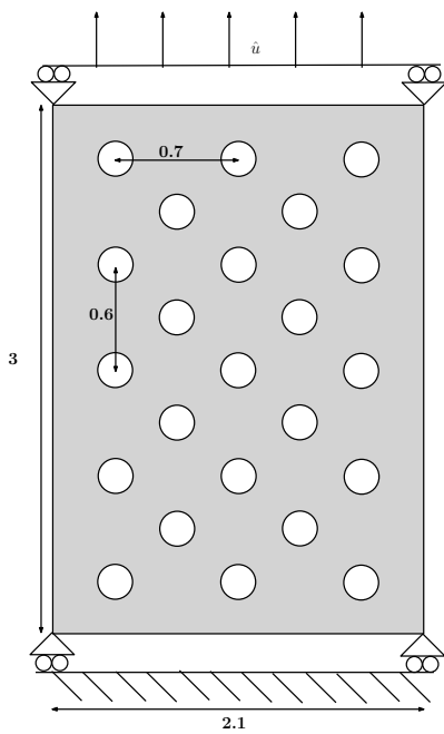
Figure 29: Geometry in mm and boundary conditions
