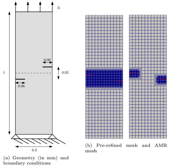
Figure 26: Fixed mesh and AMR initial mesh used for the "en-passant" sample. Red markers correspond to nodes where \hat{d} = 1 is enforced
