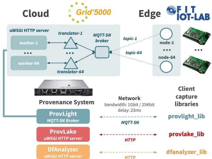
Fig. 5: Experimental setup.
