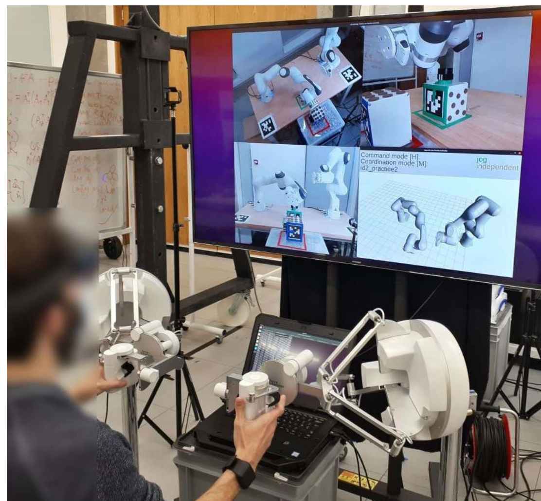
User interfaces for multi-contact teleoperation. Left : Operator commands free end-effectors' pose and triggers contact switch. Right : Remote bimanual docking and assembly task.
