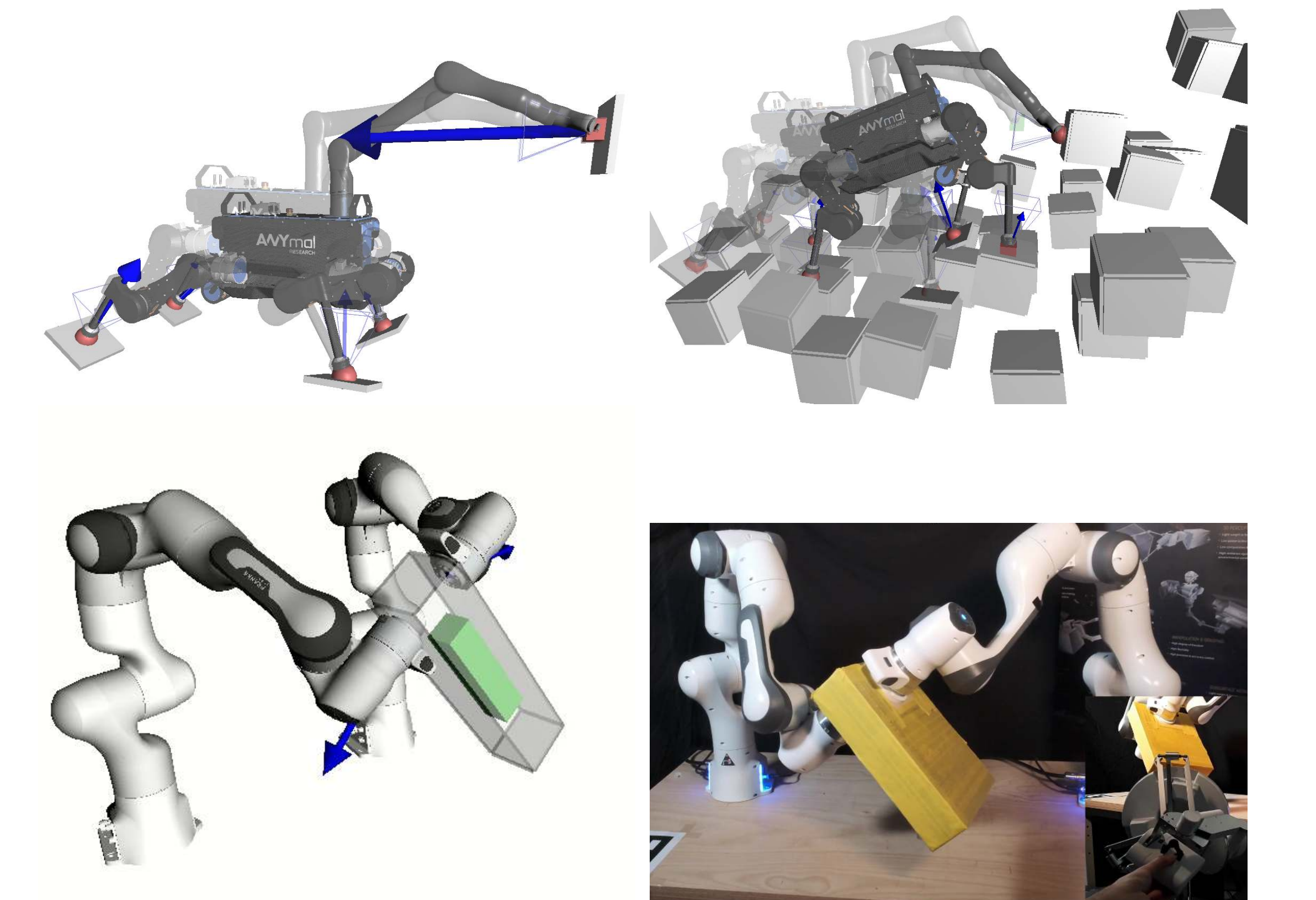
Teleoperated configurations on Valkyrie and Talos humanoid robots, on ANYmal quadruped robot and on dual arms bimanual Franka robot. Multi-contact configuration with static equilibrium, pushing tasks, locomotion on uneven terrain and manipulation of large objects.
