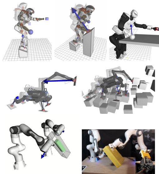
Figure 1. Multi-contact configurations computed by SEIKO during teleoperated tasks on Valkyrie and Talos humanoid robots, on ANYmal quadruped robot and on dual arms bimanual Franka robot.
