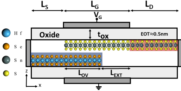
Fig. 3: Sketch of the vertical HJ TFET based on the vdW HJ of (top layer) 1T-SnS 2 and (bottom layer) 1T-HfSe 2 . Top and bottom oxides are composed of a 3.2 nm thick HfO 2 layer with an equivalent oxide thickness (EOT) of 0.5 nm. Colored areas represent doped regions.
