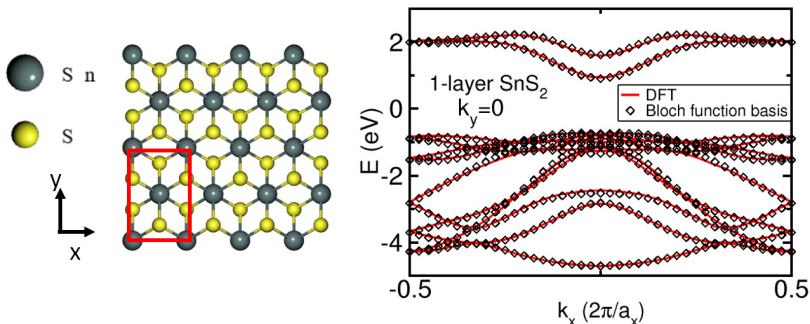
Fig. 1: (Left) orthorhombic unit cell used for transport calculations and (right) comparison of the band structure of the monolayer of SnS 2 at k_y = 0 obtained with (lines) the PW basis and (symbols) the URBF basis.
