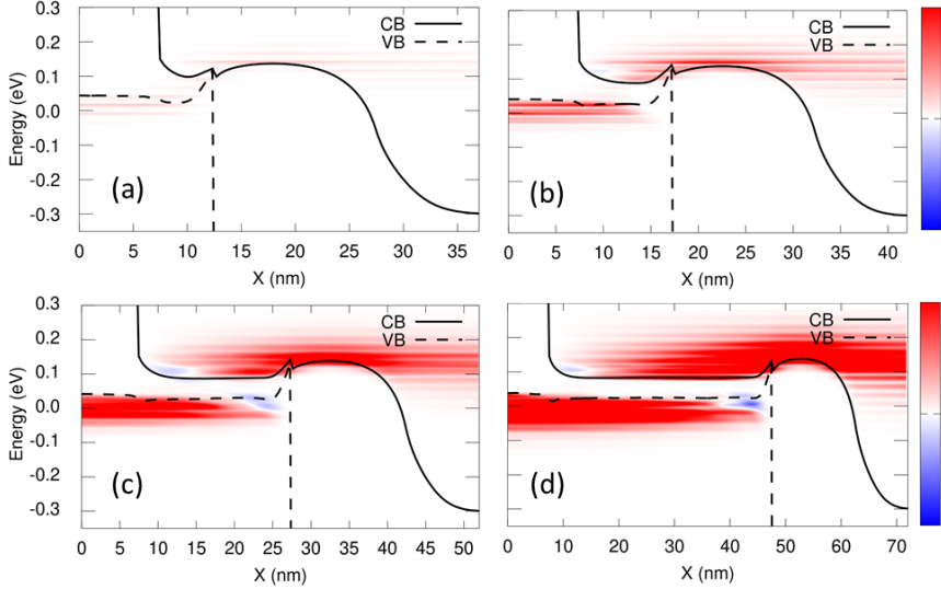
Fig. 6: (colormap) Spectral current density along the transport direction together with the VB and CB profiles at V_{GS} = 0 V and V_{DS} = 0.35 V for the vdW TFETs with (a) L_{ov} = 5 nm, (b) L_{ov} = 10 nm, (c) L_{ov} = 20 nm and (d) L_{ov} = 40 nm. Simulation parameters: D_{ac} = 5.47 eV, \tau_{op}^{-1} = 6.7 \times 10^{12} s ^{-1} , T = 300 K. The color scale is normalized with the maximum spectral current density value and ranges from -1 (blue) to 1 (red).
