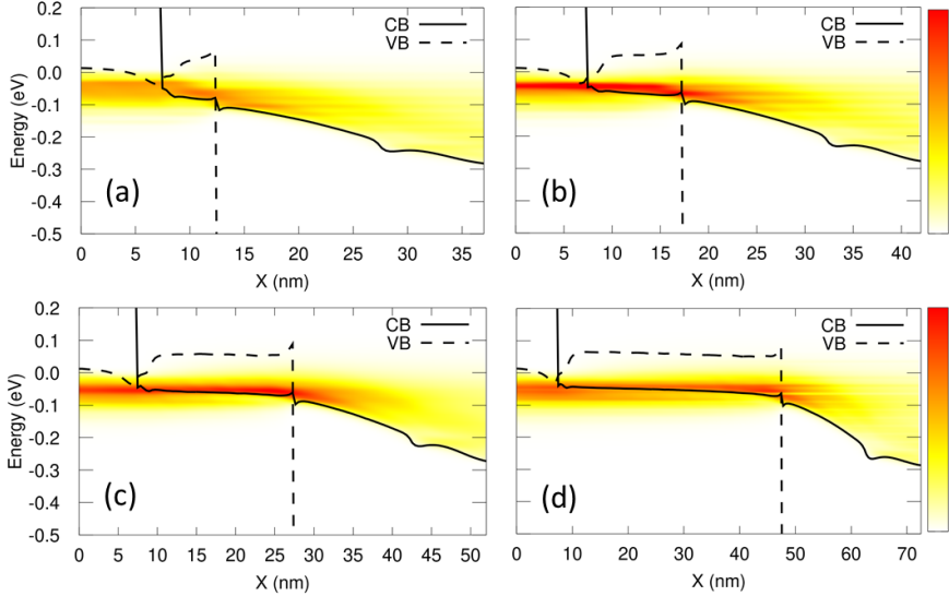
Fig. 7: (colormap) Spectral current density along the transport direction together with the VB and CB profiles at V_{GS} = 0.6 V and V_{DS} = 0.35 V for the vdW TFETs with (a) L_{ov} = 5 nm, (b) L_{ov} = 10 nm, (c) L_{ov} = 20 nm and (d) L_{ov} = 40 nm. Simulation parameters: D_{ac} = 5.47 eV, \tau_{op}^{-1} = 6.7 \times 10^{12} \text{ s}^{-1} , T = 300 K. The color scale is also normalized with respect to the maximum spectral current density value and ranges from 0 (white) to 1 (red).
