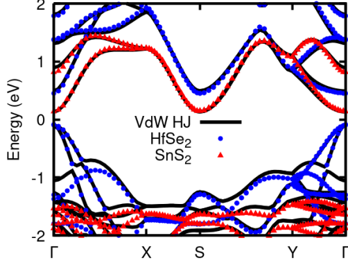
Fig. 2: Bandstructures of the monolayers of (red symbols) 1T-SnS 2 and (blue symbols) 1T-HfSe 2 , as well as of (black lines) their vdW heterostructure along the high-symmetry points of the orthorhombic unit cell used for transport calculations with cell parameters a_x = 3.726 \text{ \AA} , a_y = 6.450 \text{ \AA} .
