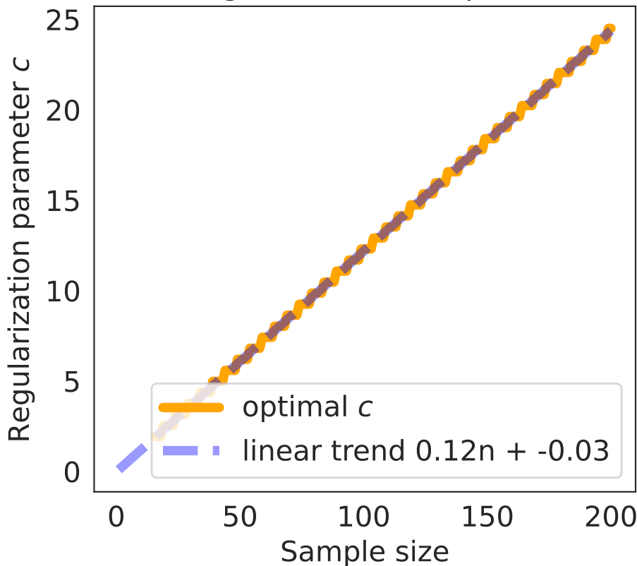
Tuning of c for N(0, 1) (averaged over 1000 repetitions)
