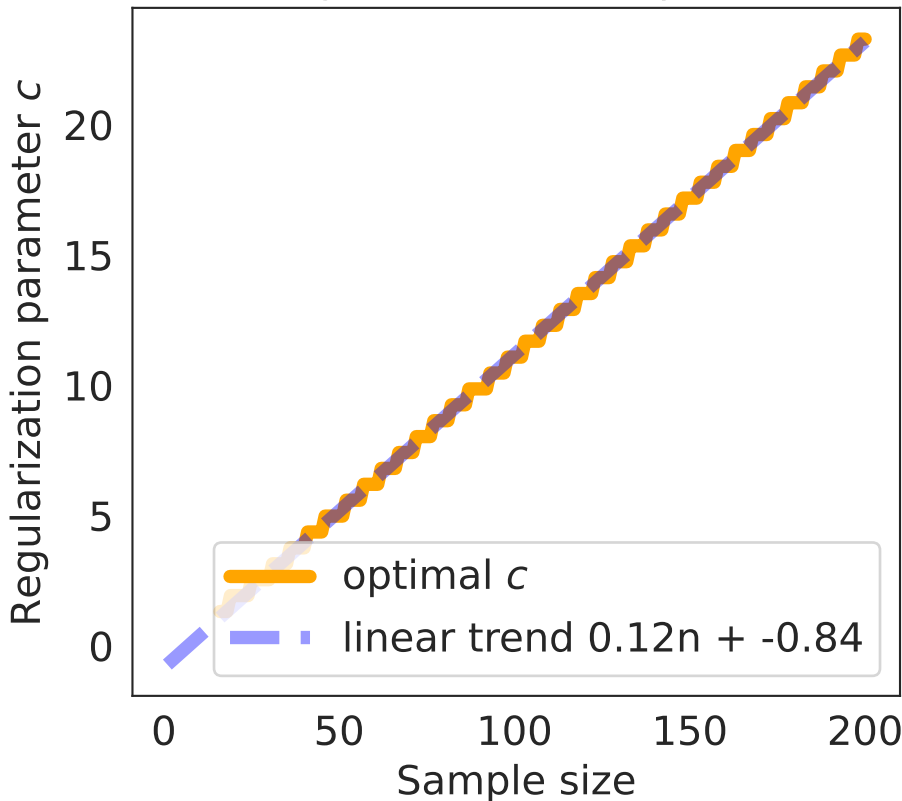
Tuning of c for E(1) (averaged over 1000 repetitions)
