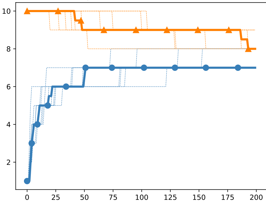
Chi Square mu:8.00, c:0.1, delta:0.01
