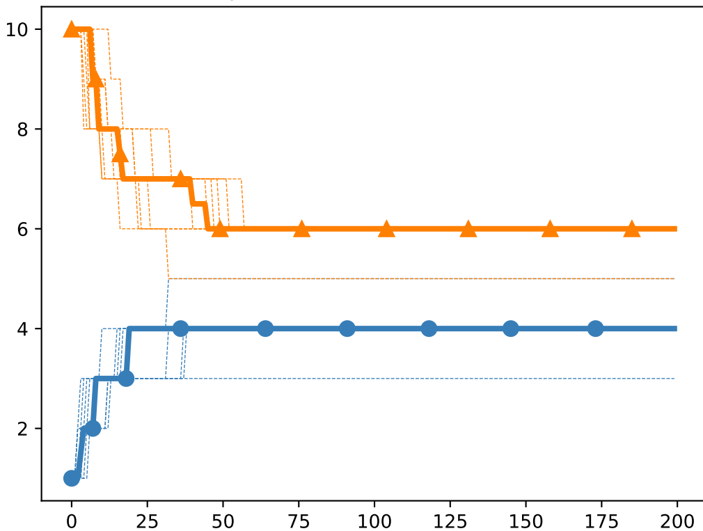
Chi Square mu:5.00, c:0.1, delta:0.01
