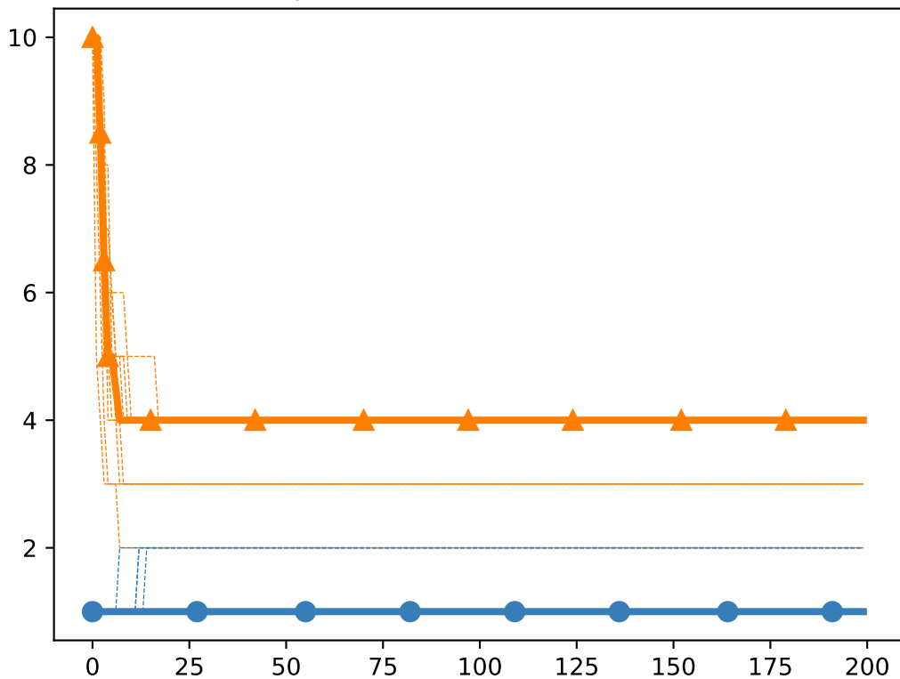
Chi Square mu:2.00, c:0.1, delta:0.01
