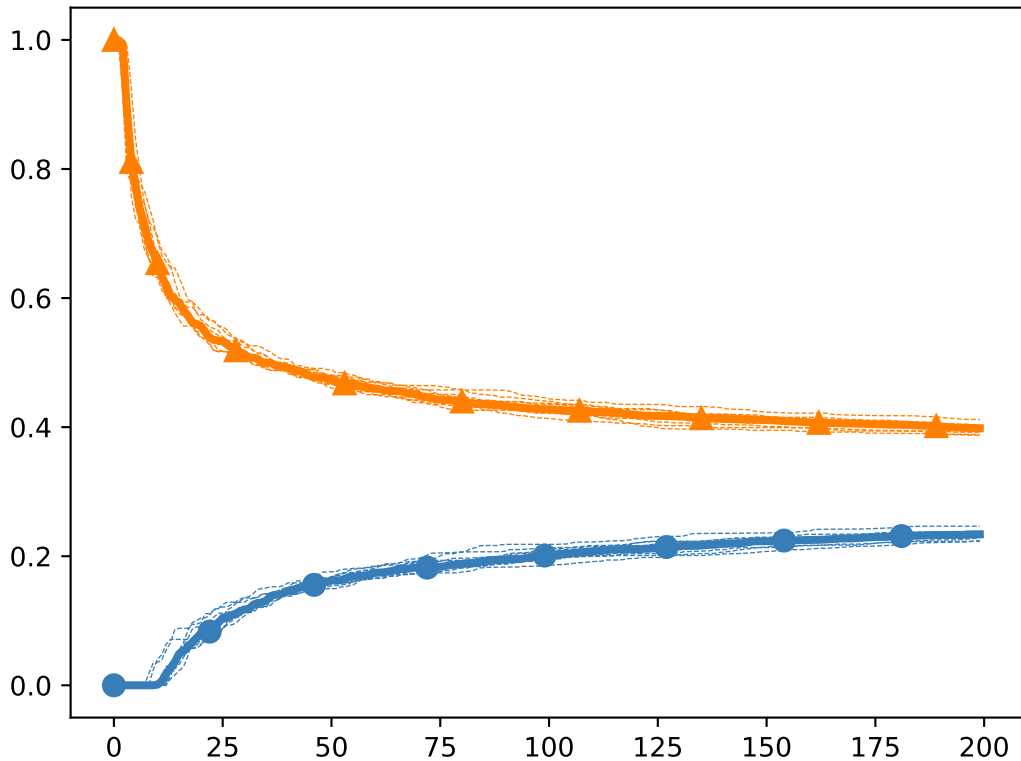
Gaussian mu:0.32, sigma2:0.10, c:0.1, delta:0.05
