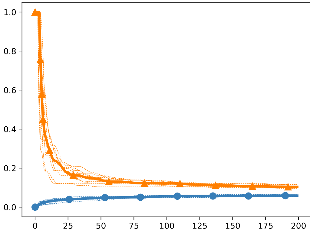
Exponential mu:0.08, c:0.1, delta:0.01
