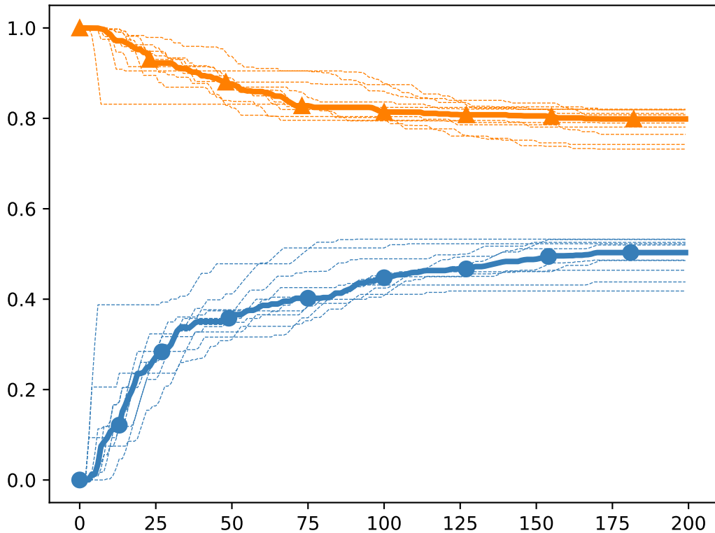
Bernoulli \mu:0.64 , c:0.1 , \delta:0.01
