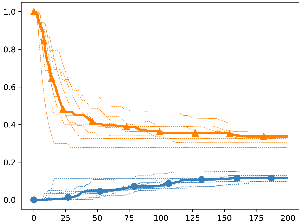
Bernoulli mu:0.22, c:1.0, delta:0.01
