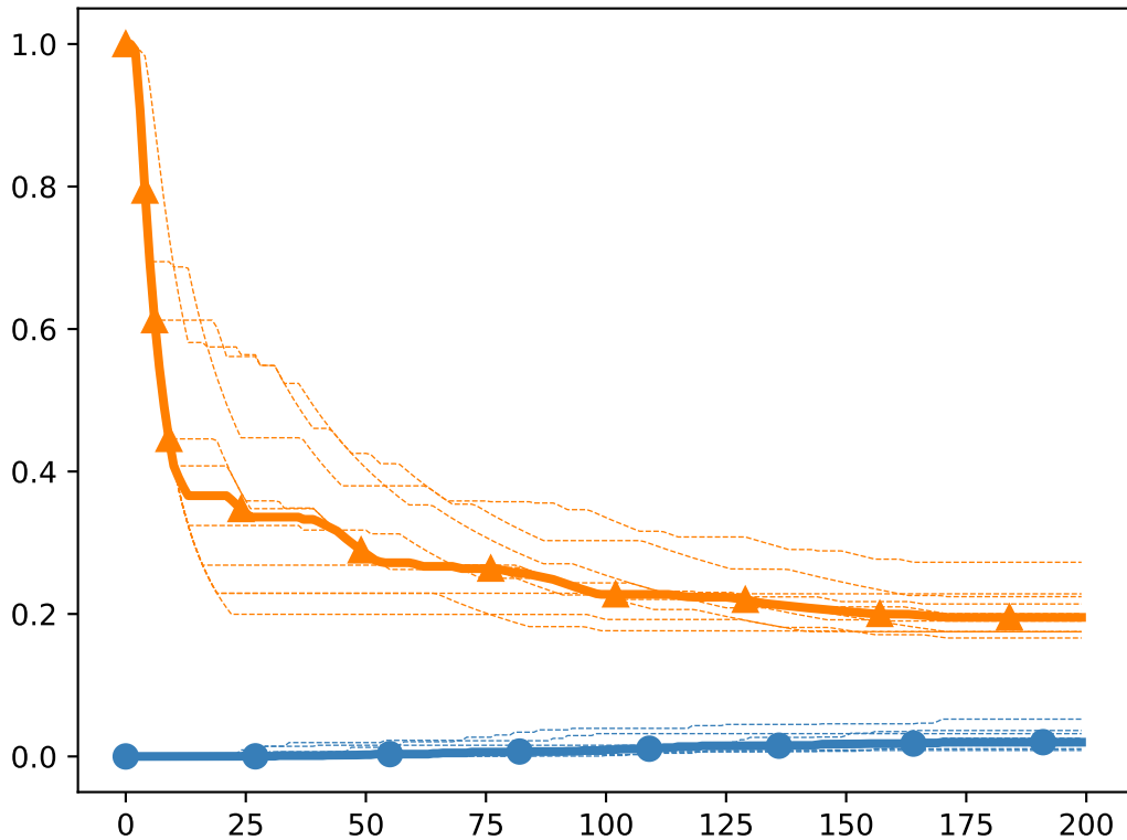
Bernoulli mu:0.10, c:0.1, delta:0.01
