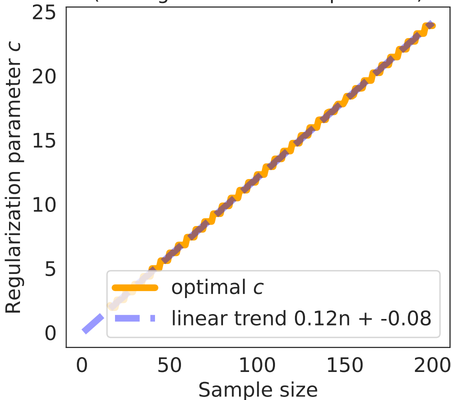
Tuning of c for \chi^2(5) (averaged over 1000 repetitions)
