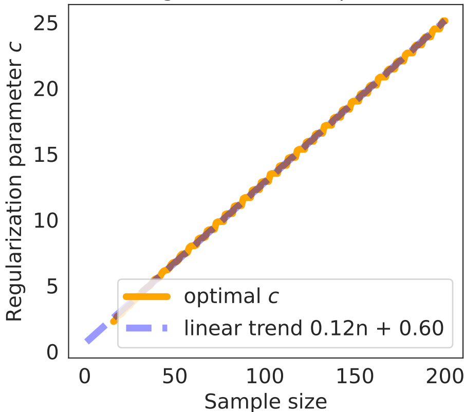
Tuning of c for B(0.7) (averaged over 1000 repetitions)
