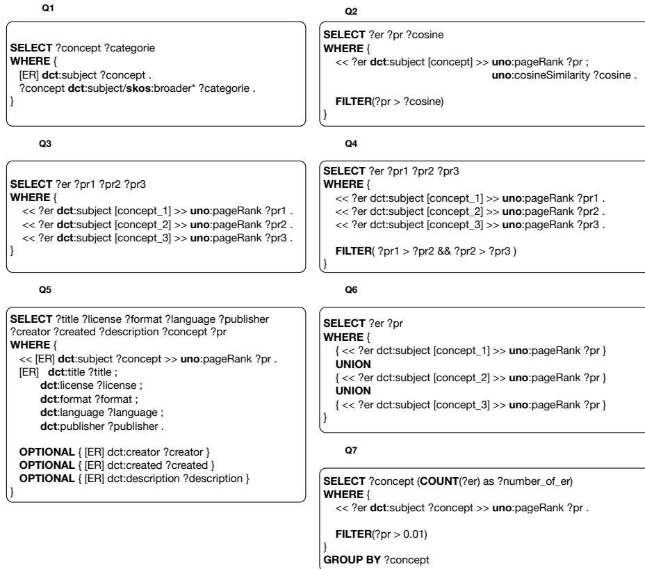
Figure 6. Query templates used for the empirical evaluation.
