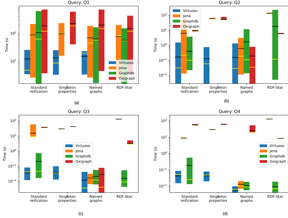
Figure 7. Execution time for queries Q1-Q4 across different data stores and reification approaches.
