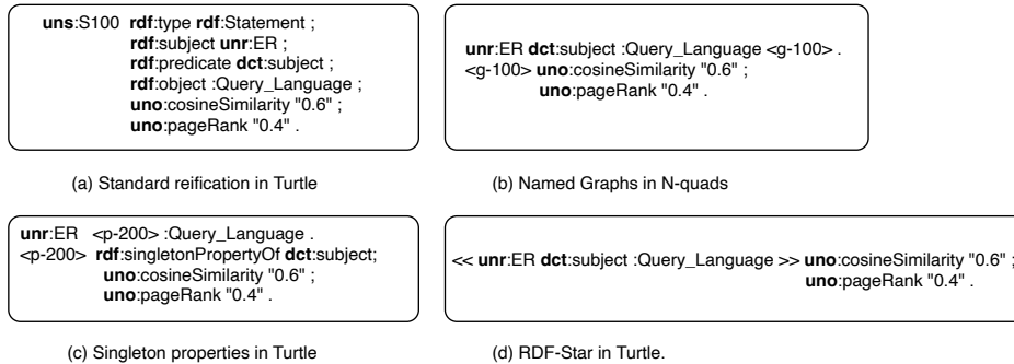
Figure 4. Syntax of the four reification models.
