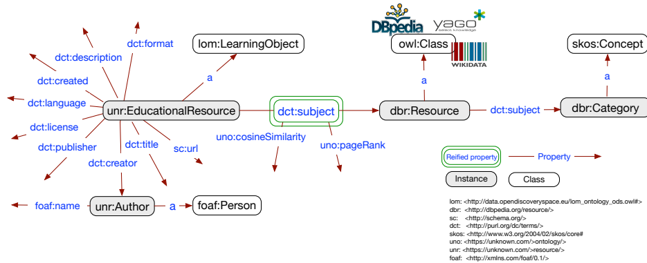
Figure 1. KG ontology.
