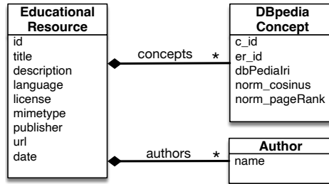
Figure 5. JSON aggregate of the source files for the RML mappings.
