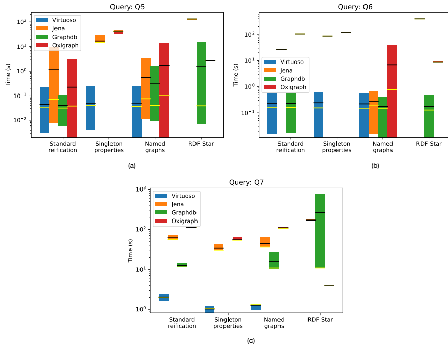
Figure 8. Execution time for queries Q5-Q7 across different data stores and reification approaches.
