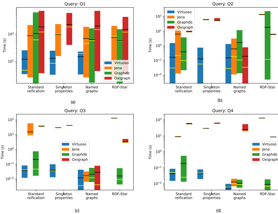
Figure 7. Execution time for queries Q1-Q4 across different data stores and reification approaches.
