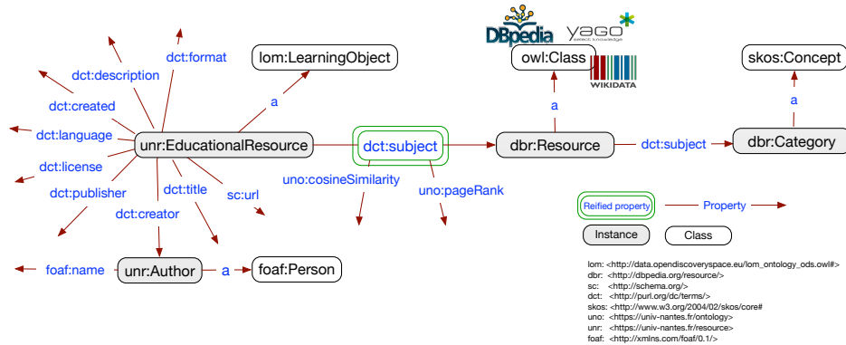
Figure 1. CLARA ontology.
