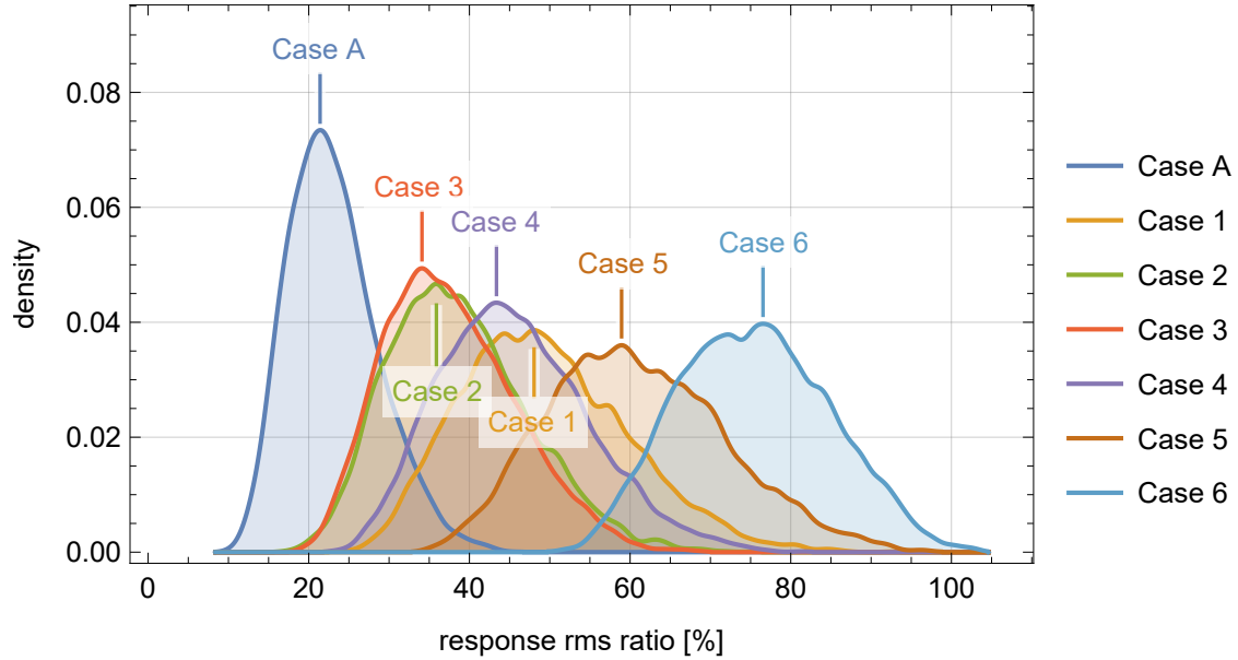
Figure 4: Histograms of the response rms ratios (controlled/passive) for the seven controlled cases
