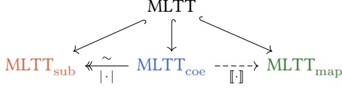
Fig. 1. Relation between \text{MLTT} , \text{MLTT}_{\text{map}} , \text{MLTT}_{\text{coe}} and \text{MLTT}_{\text{sub}} . Arrows denote type-and-conversion-preserving translations between type theories. 1
