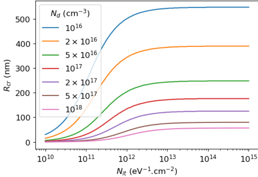
Fig. S1. Critical radius under the full depletion approximation in cylindrical coordinates as a function of surface density of states ( N_{it} ) and NW doping level ( N_d ).
