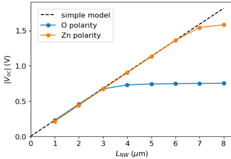
Fig. 9 Comparison of the length-dependent |V_{OC}| saturation obtained with FEM simulations for O-polar and Zn-polar crystalline orientations of the NW in a VING unit cell. Note that V_{OC} is positive with O-polar orientation and negative with Zn-polar orientation. NW radius equal to 50 nm, press action from 0 MPa to -1 MPa.
