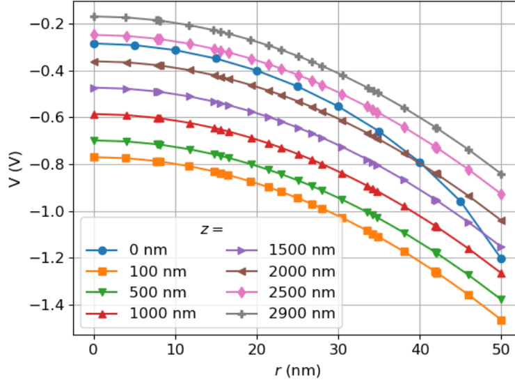
Fig. S3. Electric potential across the NW at different positions z , as obtained from FEM simulations, for O-polar orientation. We considered R = 50 nm, N_d = 5 \times 10^{17} cm ^{-3} , N_{it} = 10^{13} eV ^{-1} cm ^{-2} , L = 3 \mu m (before saturation). Here, z=0 corresponds to NW bottom (top of seed layer).
