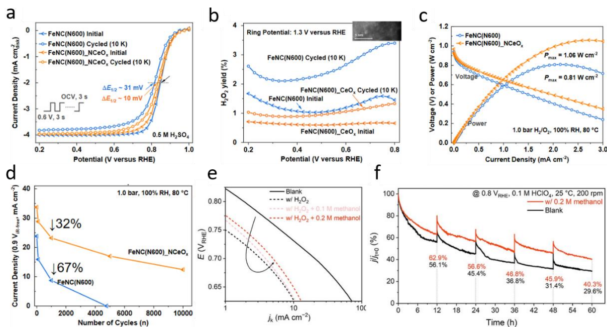
Figure 28. a) Durability of a Fe-N-C catalyst modified by N-doped \text{CeO}_x nanoparticles after ORR staircase potential steps of 0.025 V at intervals of 25 s from 1.0 to 0.0 V vs. RHE in \text{O}_2 -saturated 0.5 M \text{H}_2\text{SO}_4 at 25°C and b) associated \text{H}_2\text{O}_2 yields measured with RRDE (catalysts loading = 0.6 \text{mg}_{\text{powder}} \text{cm}^{-2} ); c) Initial performances and activities in \text{H}_2/\text{O}_2 PEMFC cathode; d) Activities losses during the DoE Electrocat Durability protocol. Anode: 0.1 \text{mg cm}^{-2} Pt/C; Cathode: 2.6 \text{mg cm}^{-2} PGM-free (Fe-N-C/ \text{NCEo}_x ), 40 wt. % Nafion ionomer; Membrane: NR211; Active area: 5 \text{cm}^2 ; 100% RH, 80°C, \text{O}_2+\text{N}_2=1 bar. e) ORR Tafel plots measured before (blank) and after the \text{H}_2\text{O}_2 treatment in pH 1 solutions with \text{H}_2\text{O}_2 (without methanol, or with methanol in 0.1 or 0.2 M concentration); f) Normalized current density of the Fe-N-C catalytic layer vs. time. The potential was set at 0.8 V vs. RHE for 60 h in the presence (red curve) or absence of 0.2 M methanol in an \text{O}_2 -saturated 0.1 M \text{HClO}_4 electrolyte. Figures a, b, c, d are reprinted from Ref. 284 . Public Domain. Figures e and f, reproduced with permission from Ref. 156 Copyright [2020] American Chemical Society.
