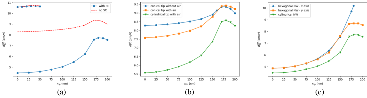
Figure 3. Simulated effective piezoelectric coefficient as a function of the position of the AFM tip across the NW surface for different simulation conditions. (a) 100 nm (top left) and 400 nm (bottom) diameter NW with (dots) and without (dashed lines) semiconducting properties in the Figure 2(a) configuration. (b) 400nm diameter NW without semiconducting properties in the configurations of Figure 2(a) (dots), 2(b) (triangles) and 2(c) (squares). (c) 400 nm diameter NW with semiconducting properties in the Figure 2(a) (triangles) and 2(d) (dots and squares) configurations. When semiconducting properties are included, N_{it}=10^{13} eV^{-1}.cm^{-2} and N_d=10^{17} cm^{-3} .
