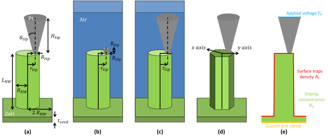
Figure 2. Schematics of the 3D numerical simulation of the deformation of a single NW by PFM within COMSOL environment in different configurations. (a) With a conical tip and without surrounding air, (b) with a cylindrical tip and with air and (c) with a conical tip, air configuration and a cylindrical NW. (d) With a conical tip, without air and with a hexagonal NW configuration. (e) Cut view of the electrical and mechanical boundary conditions.
