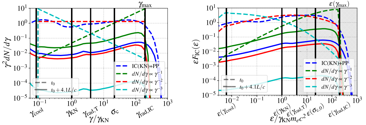
Figure 13. Left: numerical experiment wherein different initial power-law particle distributions, dN/d\gamma \propto \gamma^{-p} for p = 1, 2, and 3, are passively cooled under IC emission and pair production. All parameters are identical to the IC(KN)+PP simulation. Integration is done from time t_0 (dashed curves) to t_0 + 4.1L/c (solid curves). For reference, we present, in blue, the passive cooling of the particle distribution yielded by the IC(KN)+PP simulation (as in Fig. 12). Right: IC emission spectra corresponding to the particle distributions at left. A grey region indicates unobserved (above pair-production threshold) photon energies. After an initial-condition-dependent relaxation period, all distributions converge to an initial-condition-independent universal shape. At observable energies – that is, in the Thomson regime, \epsilon \lesssim \gamma_{KN}m_e c^2 ( \gamma \lesssim \gamma_{KN} ) – this universal shape features an approximate \gamma^{-2} power law, corresponding to \epsilon F_{IC}(\epsilon) \propto \epsilon^{0.5} . (The apparent upturn in the particle distributions at low energies is an artefact of short integration times – it results from a bulk population of cooled particles that would gradually become still colder with time, extending the \gamma^{-2} scaling to even lower energies.)
