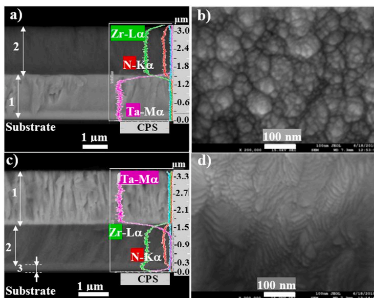
Fig. 3. SEM cross-section images and surface morphologies of N1 (a - b) and N2 (c - d) coatings, obtained on Si (100) substrate. Labels (1), (2), and (3) indicate Ta, ZrN, and Zr layers, respectively.
