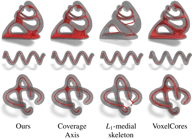
Fig. 4: Comparison with Coverage Axis, L_1 -medial skeleton and VoxelCores on standard shapes.
