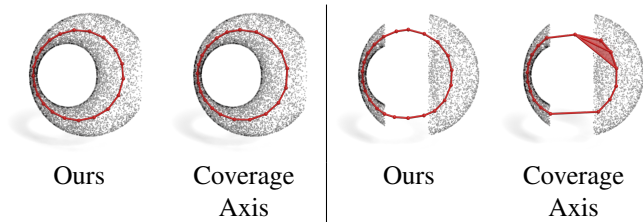
Fig. 9: Comparison with Coverage Axis on point clouds with missing data.
