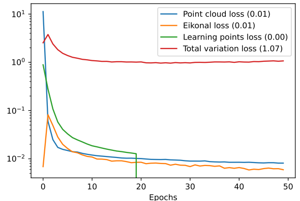
Fig. 11: Evolution of the different terms of the loss. After 20 epochs, we remove the learning points loss (Equation 5) to allow for more flexibility since in case of noise or missing data, the learning points might be inaccurate.
