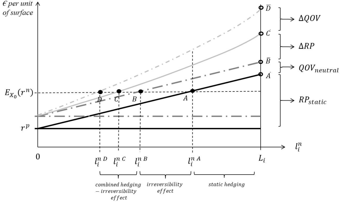
Figure 1: Effects of risk aversion, irreversibility, and farmer's hedging behavior
