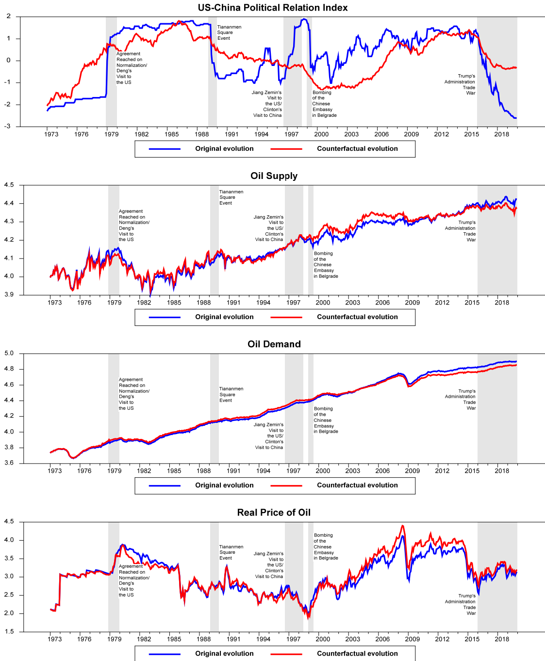
Figure 4: Counterfactual evolution
