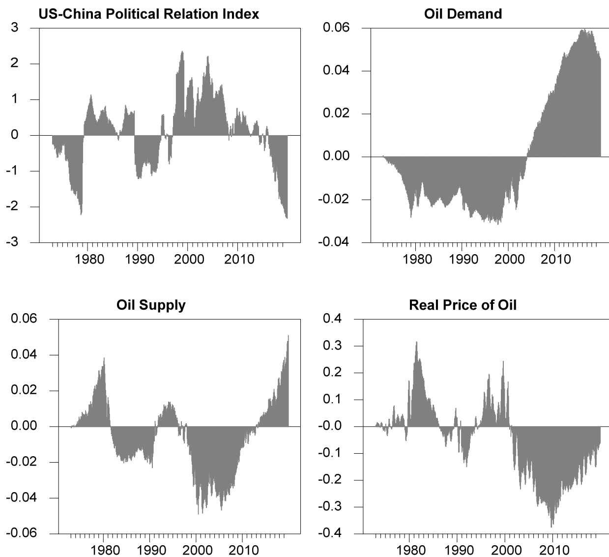
Figure 3: Historical decomposition
