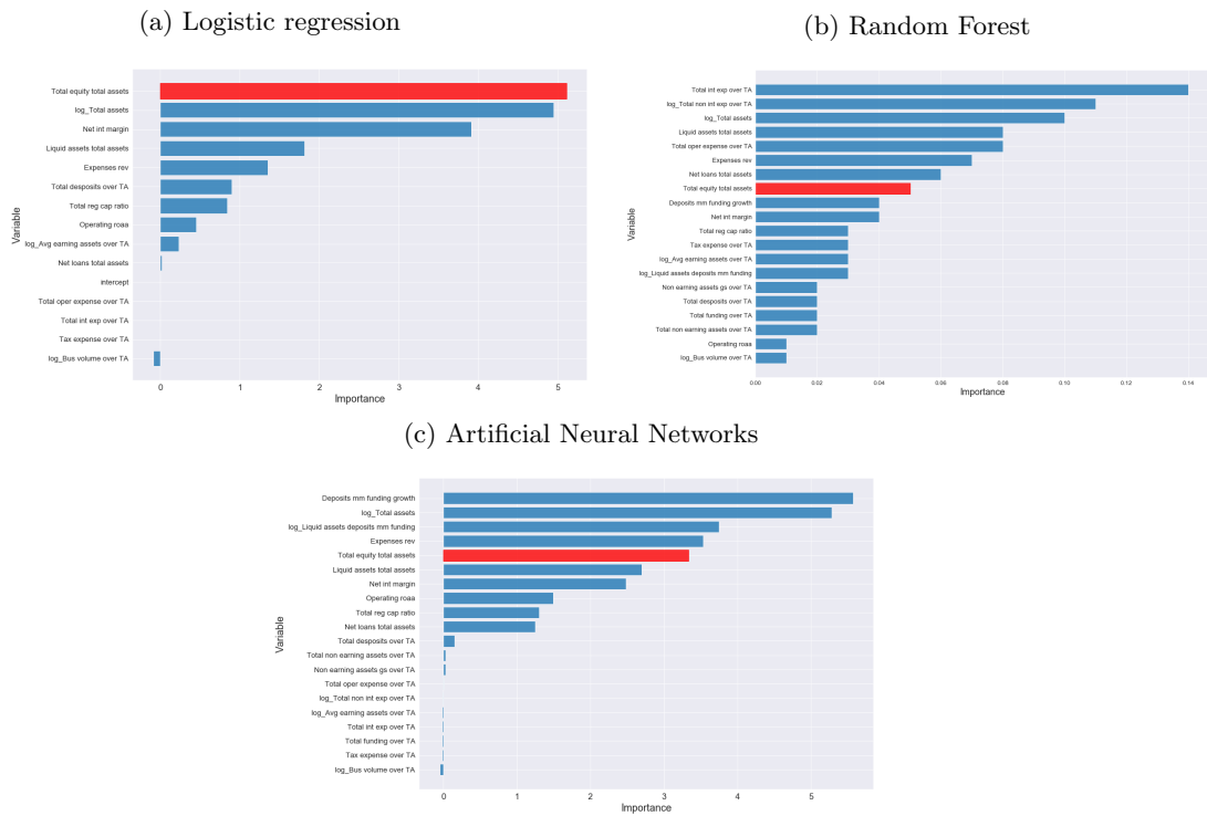
Figure 8 – Variables relative importance - Europe
