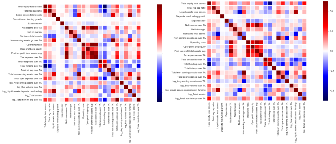
Figure 4 – Correlation hitmap - US versus Europe
