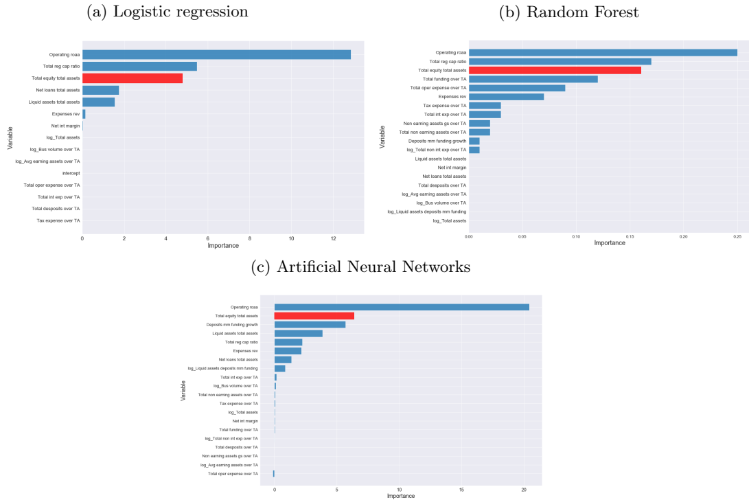
Figure 5 – Variables’ relative importance - US
