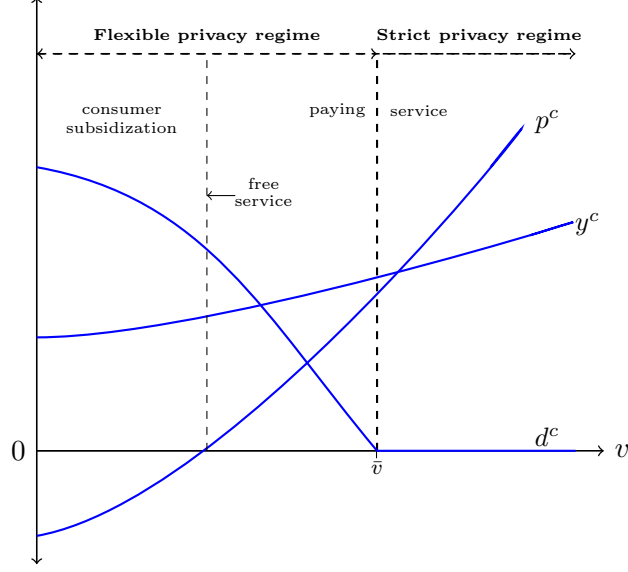
Figure 2: Equilibrium in single-homing duopoly
