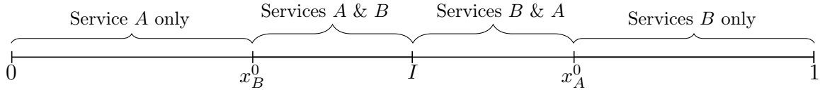
Figure 3: Demand composition with multi-homing
