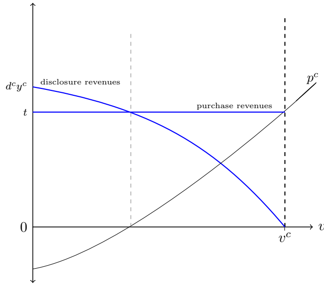
Figure 1: Pricing trade-off in flexible-privacy regime
