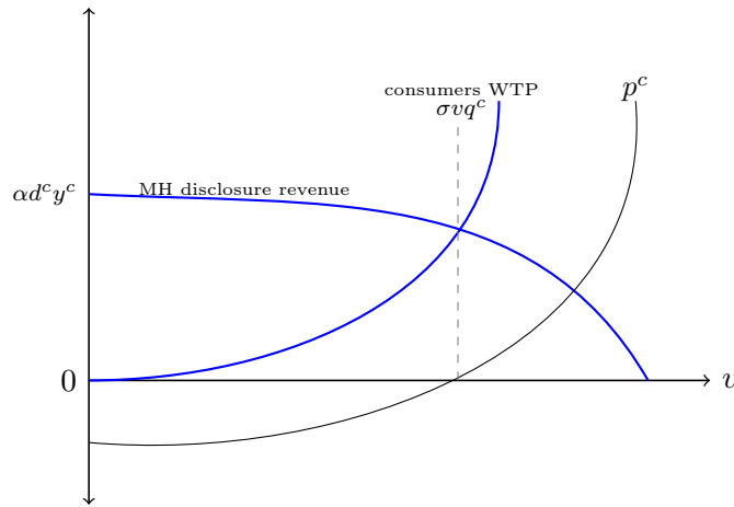
Figure 4: Pricing trade-off with MH
