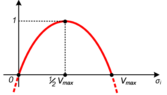
Fig. 2. Graphical representation of the set W_{i0}
