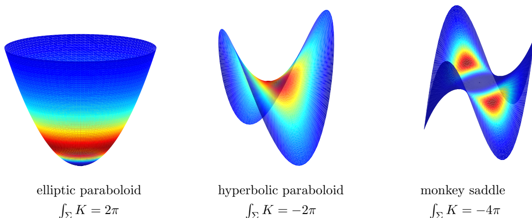
Figure 7: Examples of surfaces and their total Gauss curvatures.
