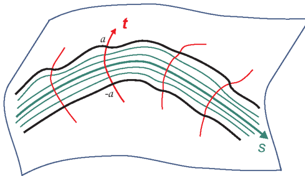
Figure 4: Strips on surfaces ( d_1 = 1 = d_2 ).
