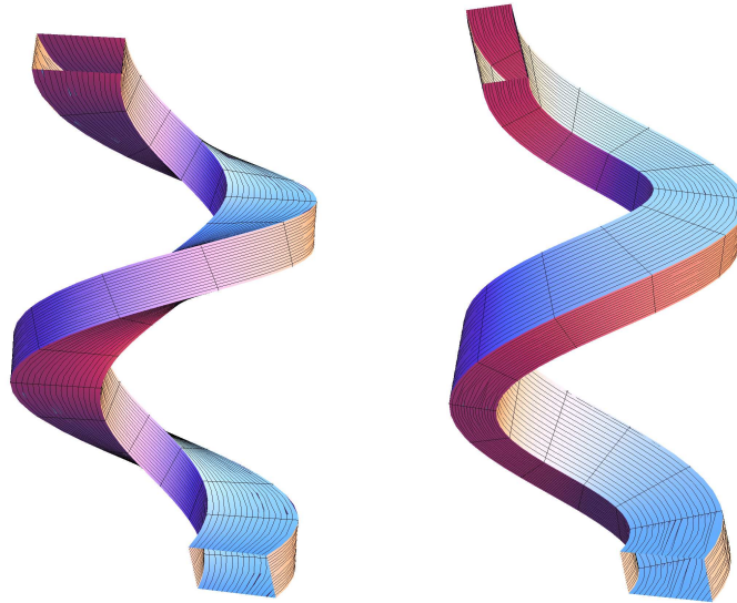
Figure 9: A tube of rectangular cross-section about a helix obtained by using the Frenet frame (left) or the relatively parallel frame (right).
