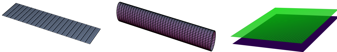
Figure 6: Straight strips, tubes and layers, respectively.
