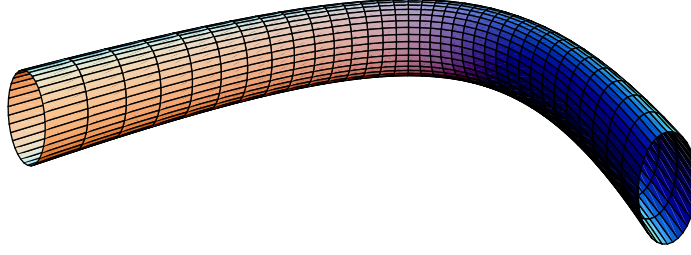
Figure 11: A purely bent tube.
