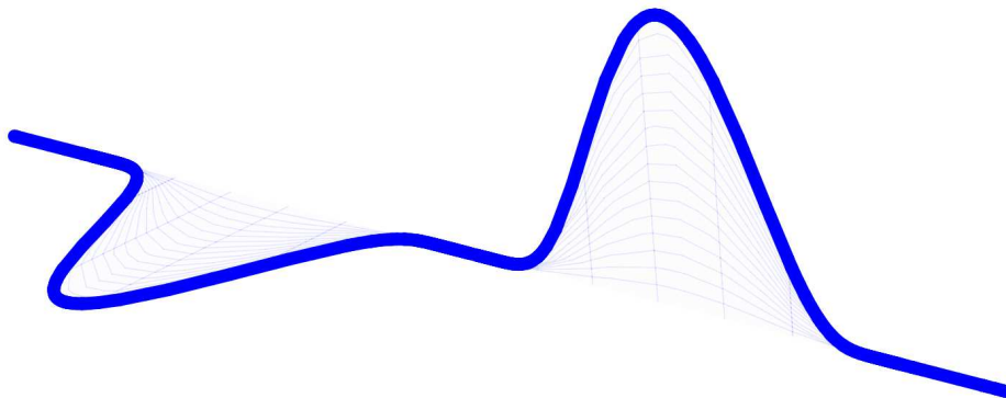
Figure 8: A curve without the Frenet frame.
