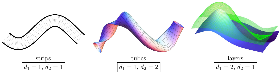
Figure 3: Euclidean tubes in low dimensions.
