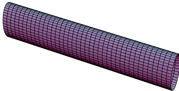
Figure 10: A straight tube.
