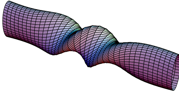
Figure 12: A purely twisted tube.
