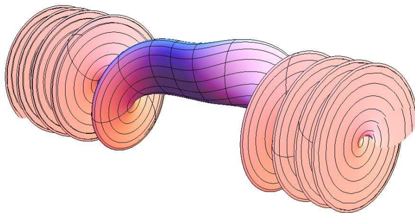
Figure 13: A tube with diverging twisting with purely discrete spectrum (Theorem 2.12).
