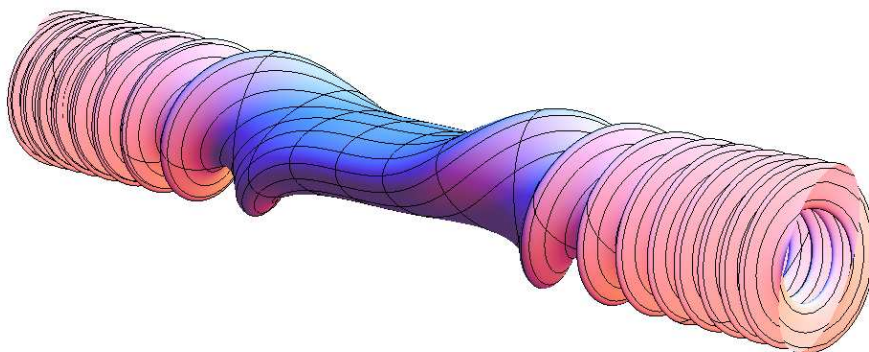
Figure 14: A tube with diverging twisting with a non-empty essential spectrum (Theorem 2.13).
