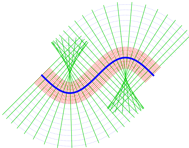
Figure 2: A Euclidean two-dimensional tube (red) constructed by means of transverse geodesics (green) emanating from the base curve (blue). A smallness restriction on the tube radius a must be imposed, in order to avoid “local self-intersections”.
