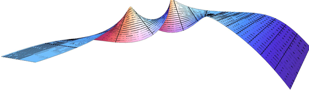
Figure 5: Strips on ruled surfaces as twisted strips.
