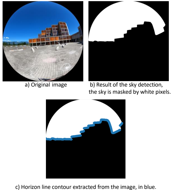
Fig. 3: Contour extraction
