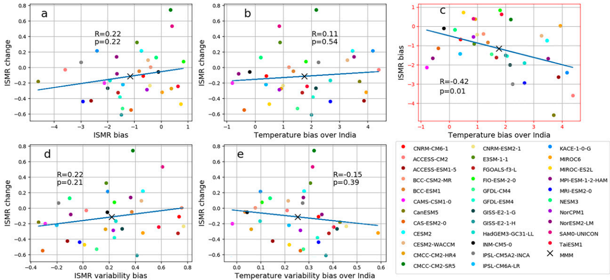
FIG. 3. Scatterplots of ISMR change ( \text{mm day}^{-1} ), respectively, with (a) mean ISMR bias ( \text{mm day}^{-1} ), (b) mean temperature bias over India (K), (d) ISMR standard deviation bias ( \text{mm day}^{-1} ), and (e) temperature standard deviation bias over India (K). Temperature biases are calculated over India, which corresponds to the same domain as the one used for ISMR. Temporal standard deviation in (d) and (e) is computed for each individual historical member and averaged for each model in case of several members. (c) Scatterplot of mean ISMR bias and mean surface temperature bias over India to illustrate local interaction between temperature and precipitation bias over India. The correlation and its associated p value for each pair of model series are indicated in each panel. The red outline means that the correlation is significant at the 95% confidence level ( p < 0.05 ). Crosses indicate the MMM position in each scatterplot.
