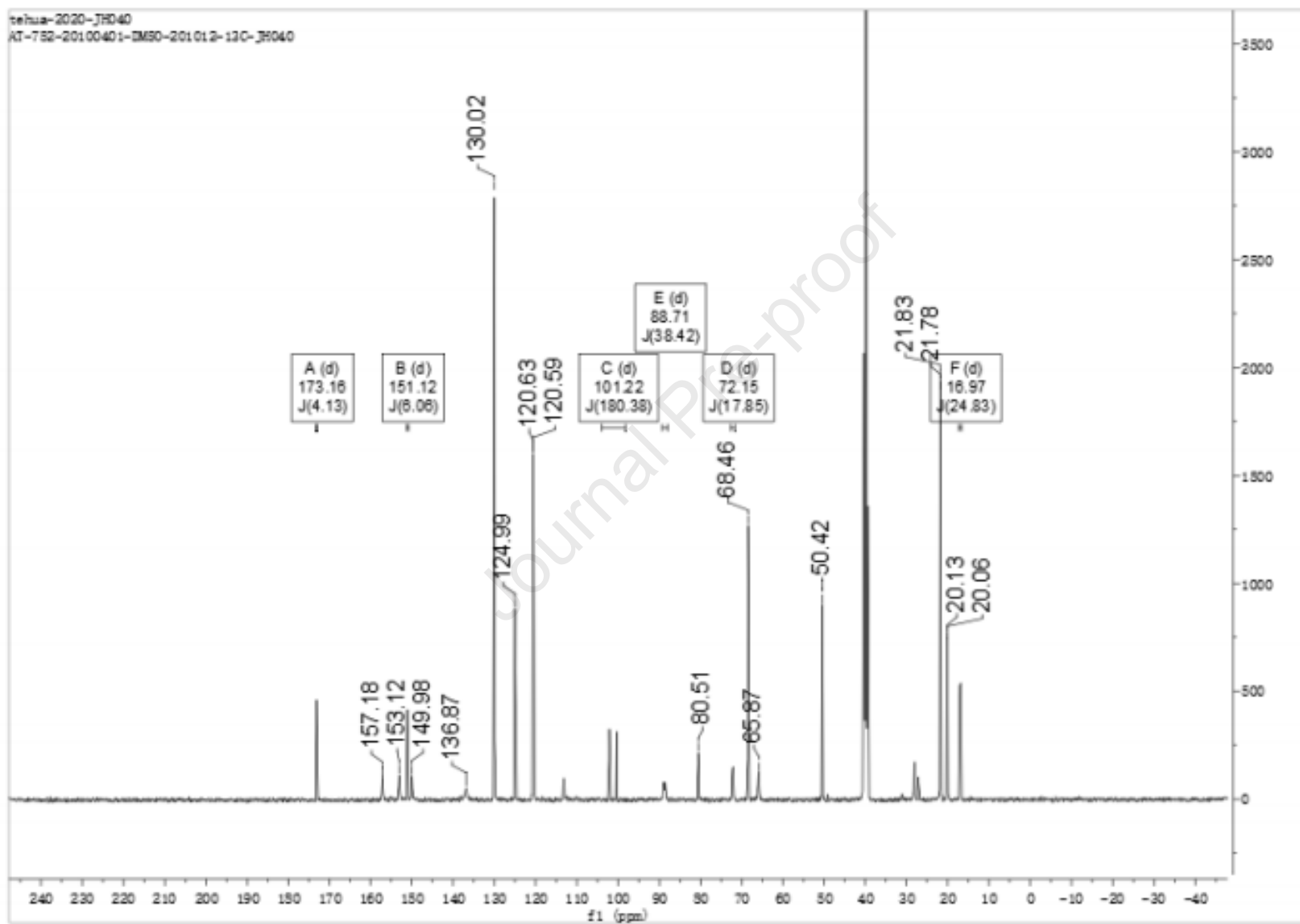
Figure 7: AT-752 Structure Elucidation— ^{13}\text{C} -NMR (Full Spectrum)
