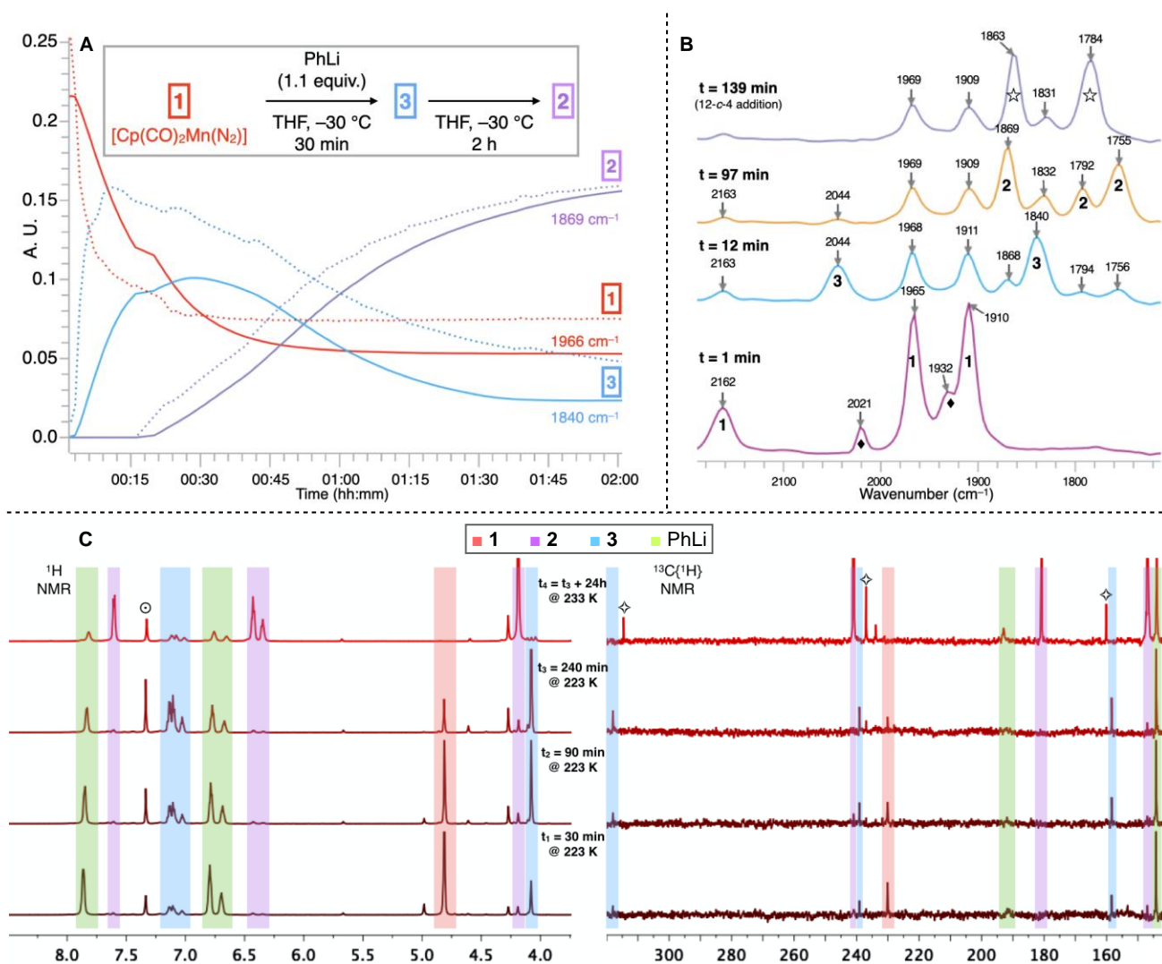
Figure 2. A) Smoothed (plain lines) and raw (dotted lines) kinetic plots of the reaction of [Cp(CO) _2 Mn(N _2 )] (1) with PhLi (1.1 equiv., THF, ca. -30^\circ\text{C} ) showing the absorbance of the most intense CO stretching band of the three main species detected by real-time IR monitoring. B) IR spectra recorded at different times of the reaction. \blacklozenge [CpMn(CO) _3 ] present in the starting material; \star 2, separated ion pair. C) Stacked spectra of ^1\text{H} - (left, 600 MHz) and ^{13}\text{C}\{^1\text{H}\} -NMR (right, 150 MHz) monitoring in THF- d_6 at low temperature focusing on the Cp/aromatic and carbonyl regions, respectively. \ominus C _6 H _6 ; \diamond [Cp(CO) _2 MnCOPh]Li (4).
