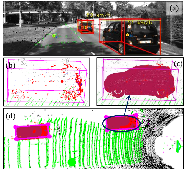
Fig. 1. In our SLAM system we track object (here cars) moving in the scene. We show here (a) a frame with tracked cars, their speed and re-projected bounding boxes. (b) the bounding box and clustered LiDAR points (red) for the closest car. (c) the reconstruction of the car, using the approach of DSP-SLAM [3]. (d) the map seen from above, with LiDAR points (black), road LiDAR points (green), tracked cars and the camera frustum (right).
