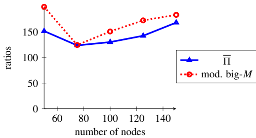
(b) Using HiGHS for the MILPs.
