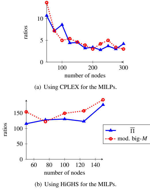
Figure 1: Geometric averages of the solution times obtained using Theorem 2 divided by those of formulations mod. big-M and ( \bar{\Pi} ).
