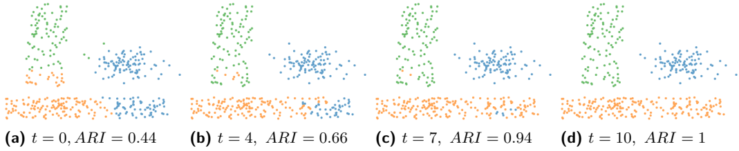
■ Figure 3 Illustration of IAC with ( \alpha = 20\% , \beta = 30\% ) over 10 iterations on lsun dataset, starting from a KMEANS partition (Fig. 3a). Subsequent figures show the evolution of the partition after t iterations of IAC with NPU. Adjusted Rand Index with ground truth is reported on each figure.
