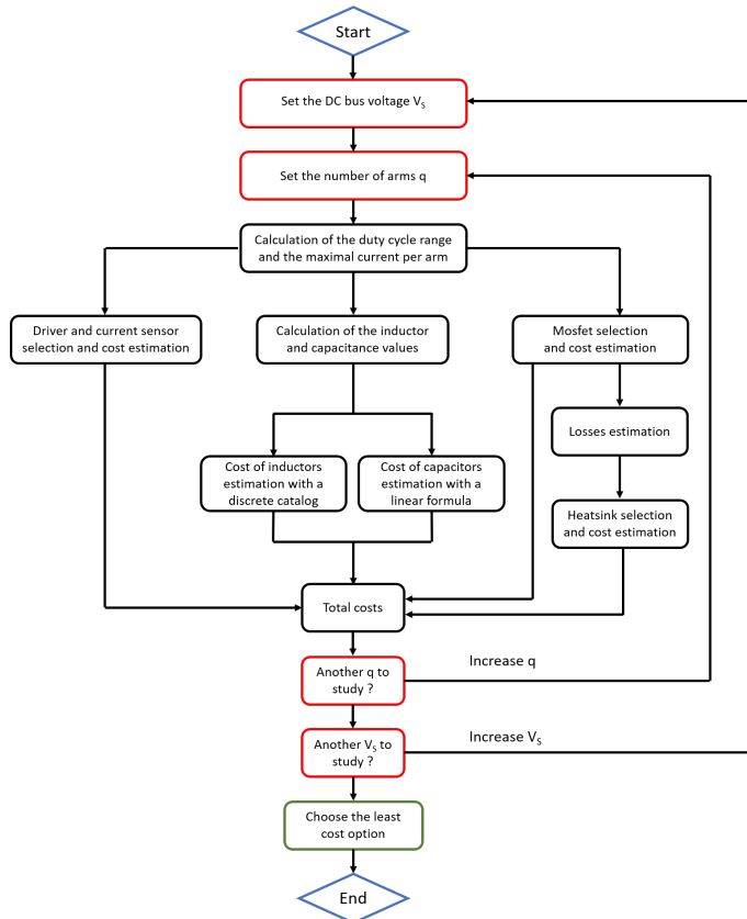
FIG. 4. Flowchart of the exhaustive search algorithm.
