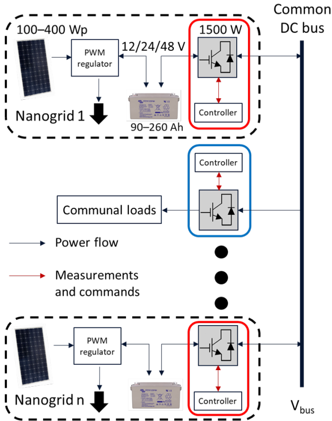
FIG. 2. Topology of the proposed microgrid.
