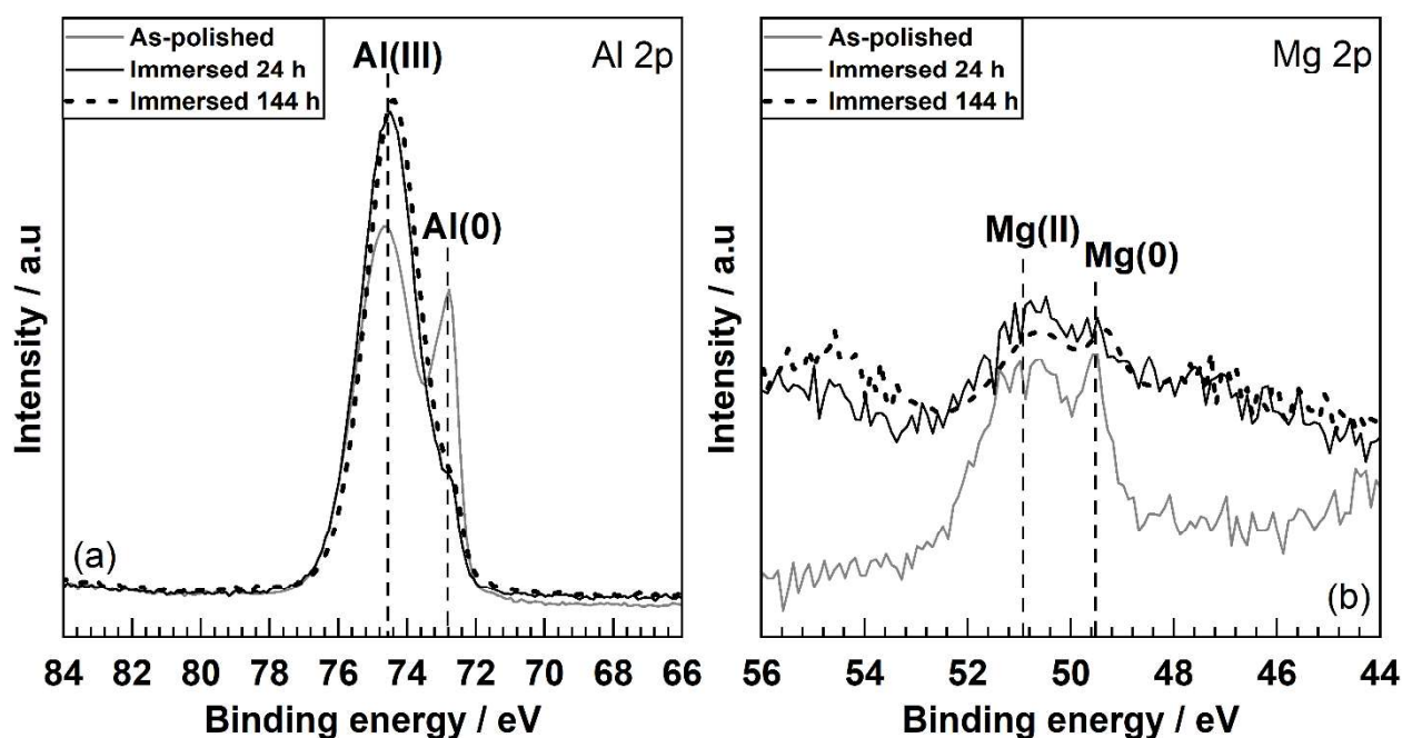
Figure 6. XPS analyses of the 1 mm L-LT samples immersed in 0.1 M Na 2 SO 4 + 0.001 M NaCl for 24 h and 144 h. Results obtained for the as-polished 1 mm L-LT sample are reported for comparison. High resolution a) Al 2p and b) Mg 2p core level spectra.
