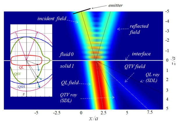
FIG. 7. (Color online) Heat map of the modulus of the stress vector for an incident monochromatic Gaussian bounded beam propagating in water ( k_0a = 170 ), which interacts with an interface between the fluid medium and an anisotropic solid medium, located at z/a = 0 (unidirectional carbon-epoxy medium, A6-axis perpendicular to the interface, incident angle equal to 21.7^\circ ; see Fig. 6). The emitting transducer is situated at (x/a = 0, z/a = -5) . The black lines represent the incident acoustic axis of the emitter transducer, the reflected, and transmitted propagation directions, such as was predicted by Snell-Descartes law (SDL). The white lines in the solid represent the direction of the energy velocity.
